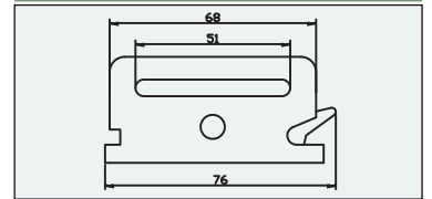
2" End Fitting F010301
