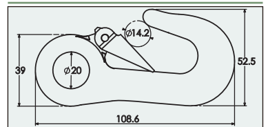
Forged Snap Hook E Series
