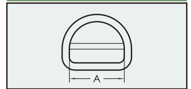
Buckle-01 F44 series
