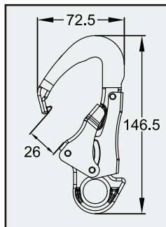
Self Locking Snap Hook RBH-M-AL-003
