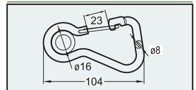
Spring Hook With Eyelet / Without Eyelet S02 Series
