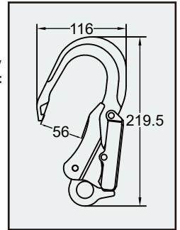
Aluminum Rebar Hook A0101 series
