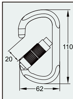
D Carabiner CBRAD-ALF-002
