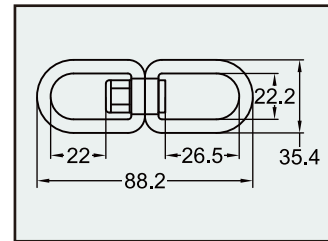
Swivel Connector - Medium I0202 series Forged Alloy Steel Yellow Zinc Plated / Chrome Plated Min. Breaking Strength: 23kN/5000lbs
