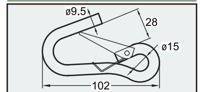
Snap Hook S11 Series
