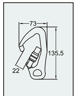
Screw Locking Snap Hook C5101 series
