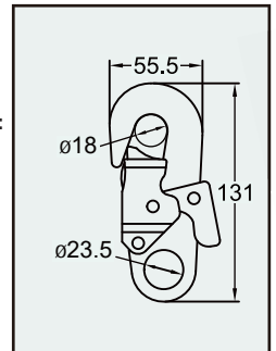
Self Locking Snap Hook A0202 series
