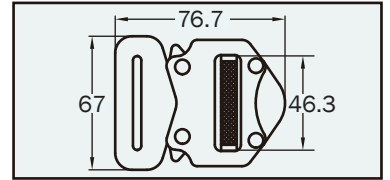
Harness Safety Buckle K0601 series
