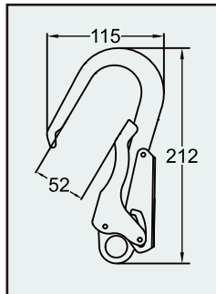
Self Locking Rebar Hook A0102 series
