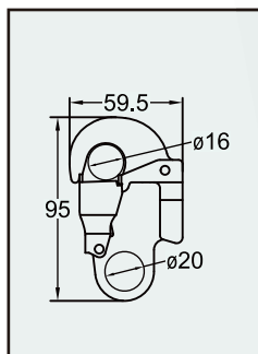
Self Locking Snap Hook A0302 series
