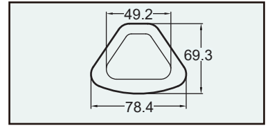
Buckle-05 F44 series
